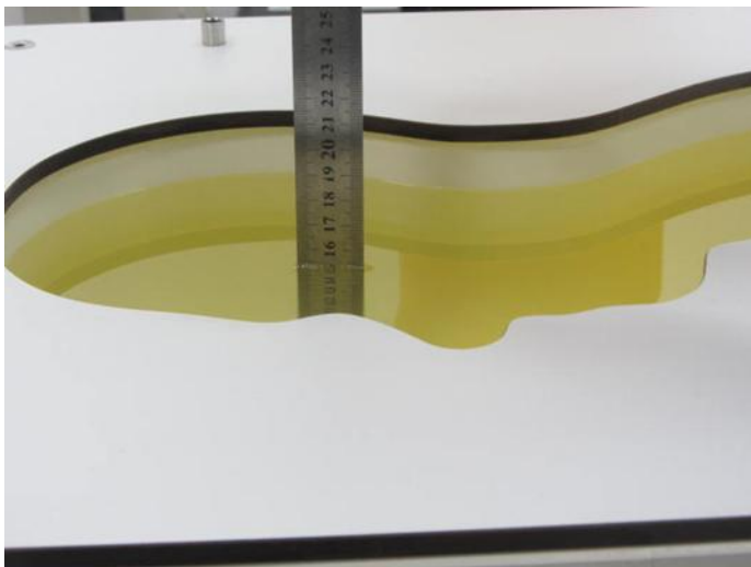
Photo 24: HSL2450MHz depth (15.0cm)
