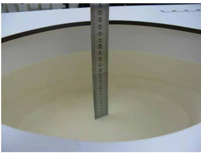
Photo 25: MSL2450MHz depth (15.1cm)
