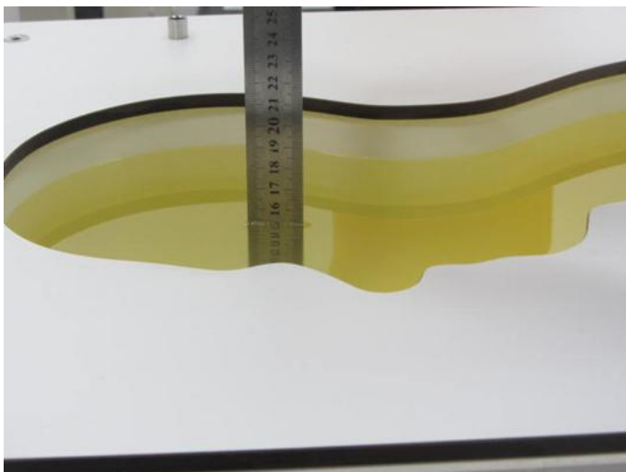
Photo 26: HSL2600MHz depth (15.0cm)
