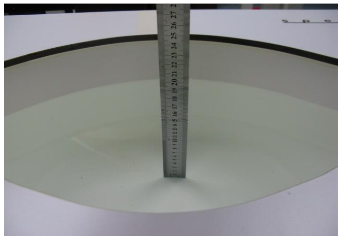
Photo 21: MSL1750MHz depth (15.1cm)
