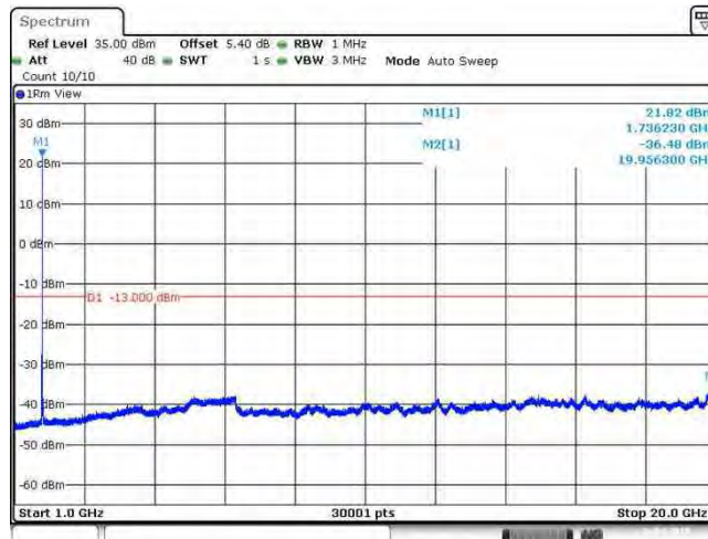
Band66_20MHz_QPSK_132322_1RB#0
