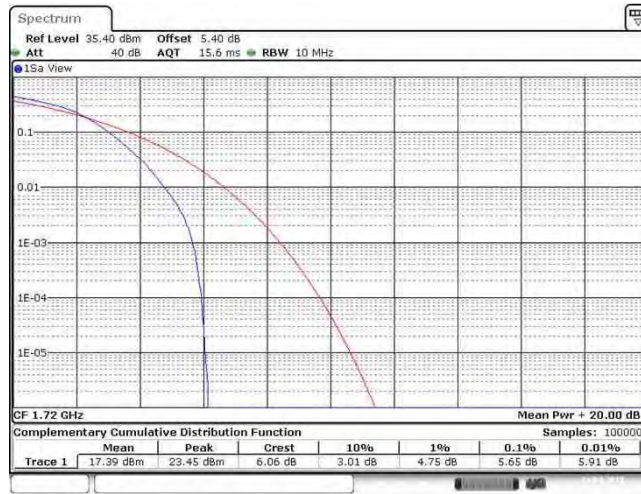
Band66_20MHz_64QAM_132322_100RB#0
