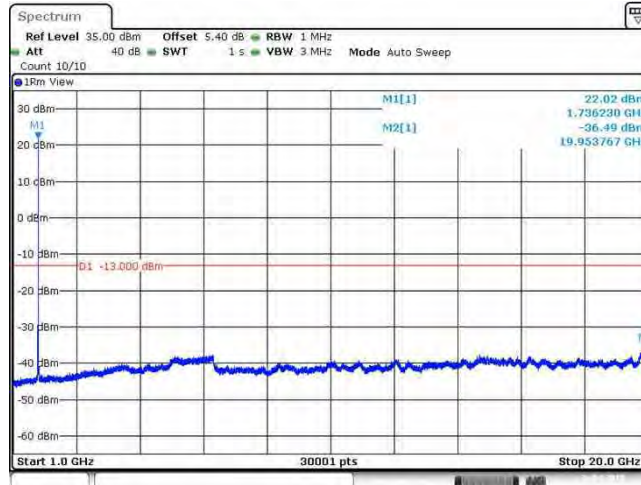
Band66_20MHz_16QAM_132322_1RB#0
