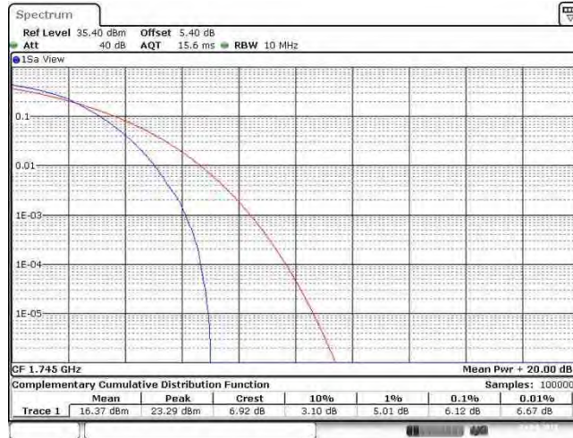
Band66_20MHz_64QAM_132322_100RB#0
