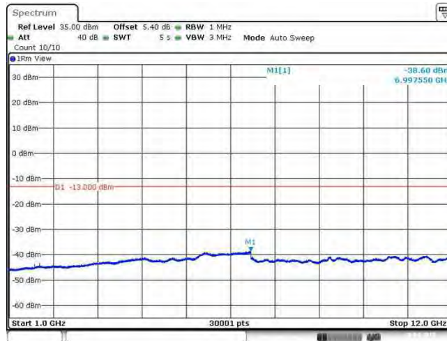
Band26_10MHz_64QAM_26740_1RB#0
