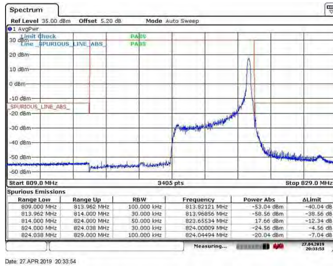
Band26_5MHz_64QAM_26765_25RB#0
