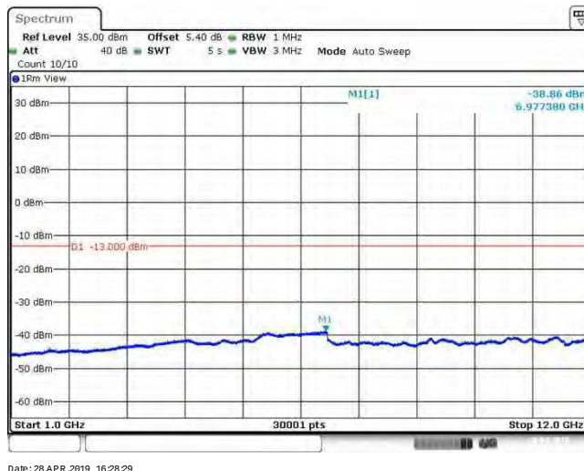
Band26_10MHz_16QAM_26740_1RB#0
