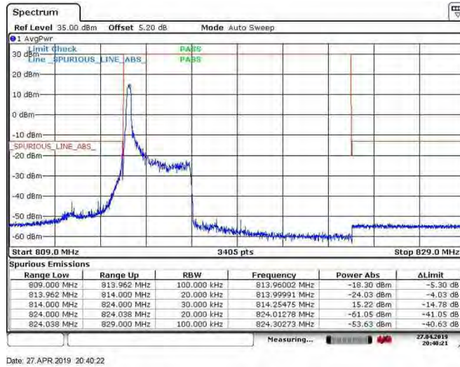
Band26_3MHz_64QAM_26705_15RB#0
