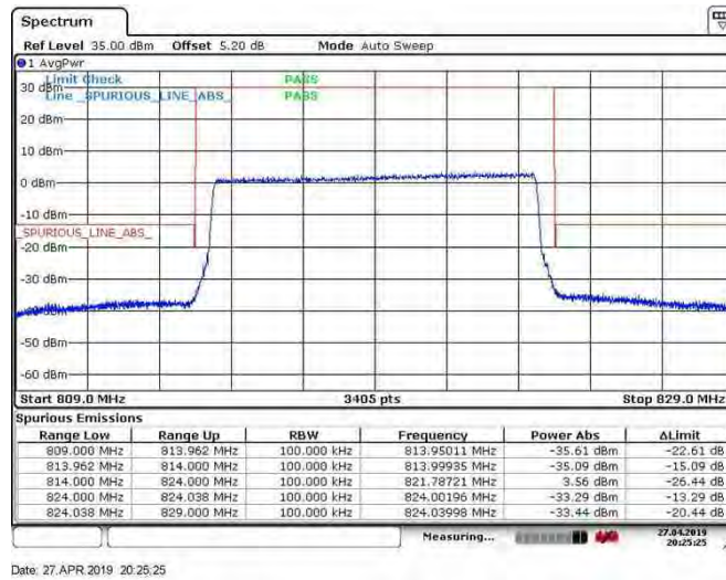
Band26_10MHz_64QAM_26740_1RB#99
