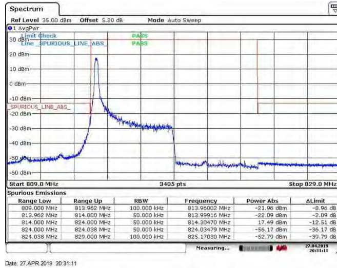
Band26_5MHz_64QAM_26715_25RB#0
