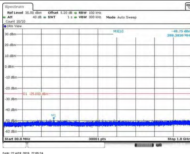
Band41_20MHz_64QAM_40140_1RB#0
