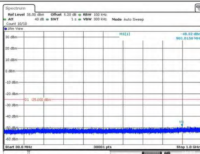
Band41_20MHz_QPSK_40140_1RB#0
