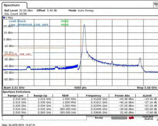
Band41_20MHz_16QAM_40140_100RB#0
