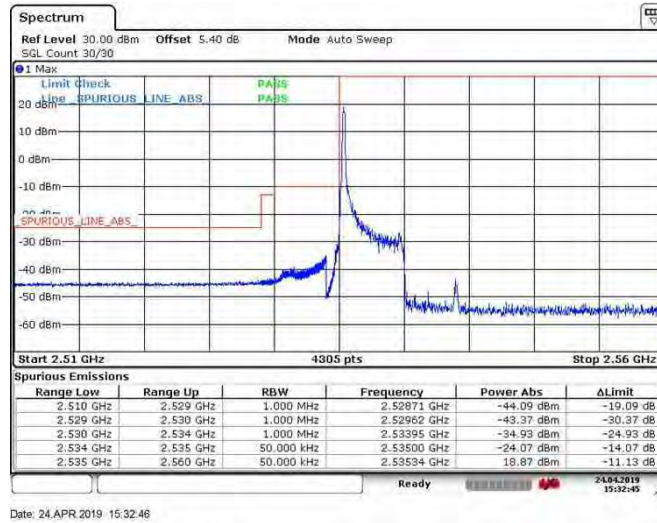
Band41_5MHz_64QAM_40065_25RB#0
