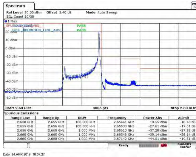
Band41_10MHz_64QAM_41190_50RB#0
