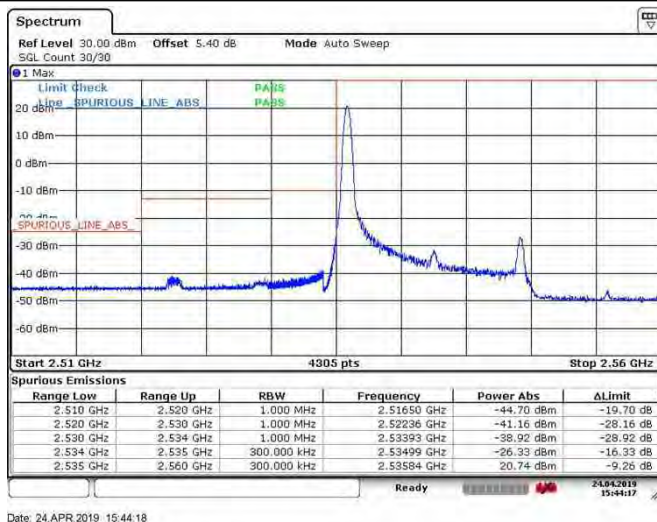
Band41_15MHz_64QAM_40115_75RB#0
