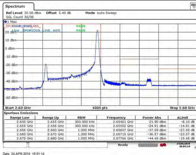
Band41_15MHz_QPSK_41165_75RB#0
