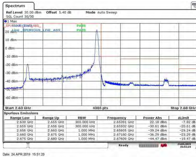
Band41_20MHz_QPSK_41140_100RB#0
