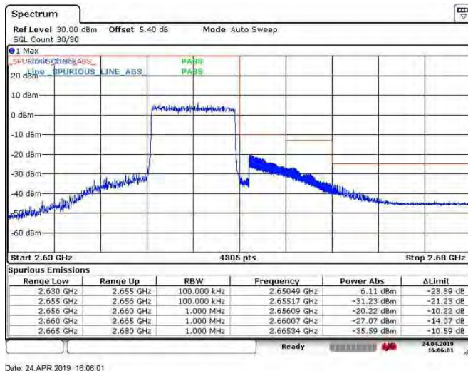
Band41_10MHz_64QAM_40090_1RB#0
