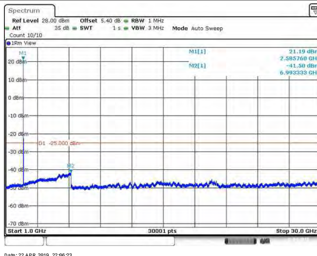
Band41_20MHz_QPSK_41140_1RB#0
