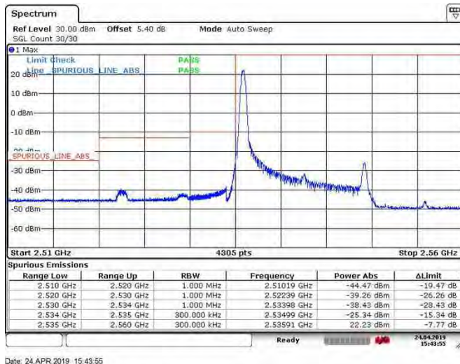
Band41_15MHz_16QAM_40115_75RB#0
