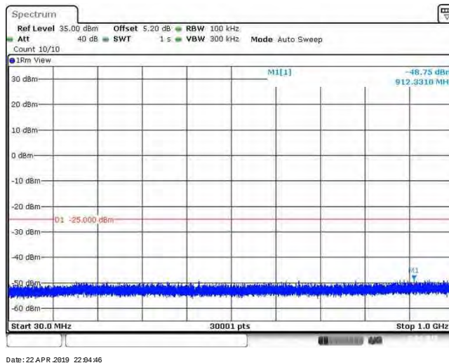
Band41_20MHz_16QAM_40140_1RB#0
