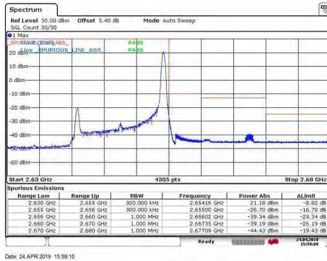
Band41_15MHz_64QAM_41165_75RB#0
