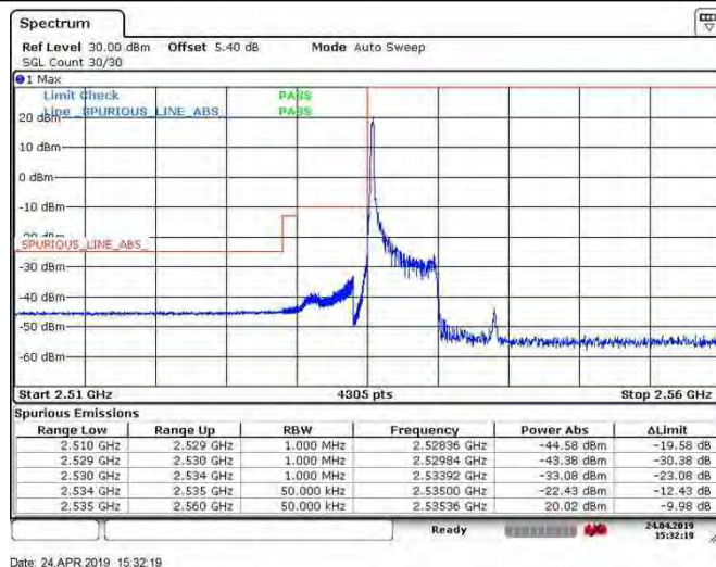
Band41_5MHz_16QAM_40065_25RB#0
