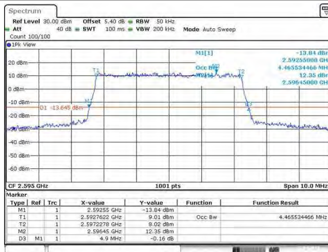
Band41_5MHz_QPSK_40640_25RB#0
