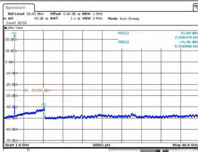
Band41_20MHz_QPSK_40140_1RB#0
