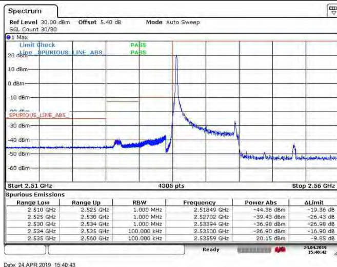
Band41_10MHz_16QAM_40090_50RB#0
