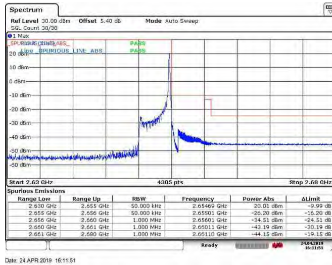
Band41_5MHz_64QAM_41215_25RB#0
