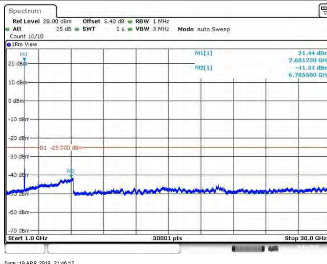
Band38_20MHz_64QAM_37850_1RB#0
