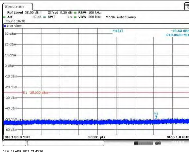
Band38_20MHz_64QAM_37850_1RB#0
