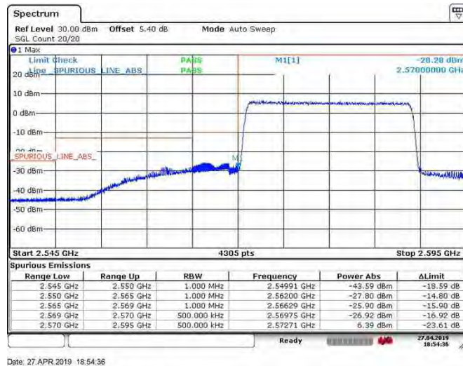
BAND38_20MHz_16QAM_38150_1RB#99
