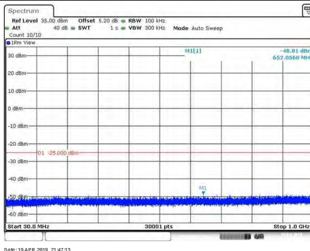
Band38_20MHz_64QAM_38150_1RB#0
