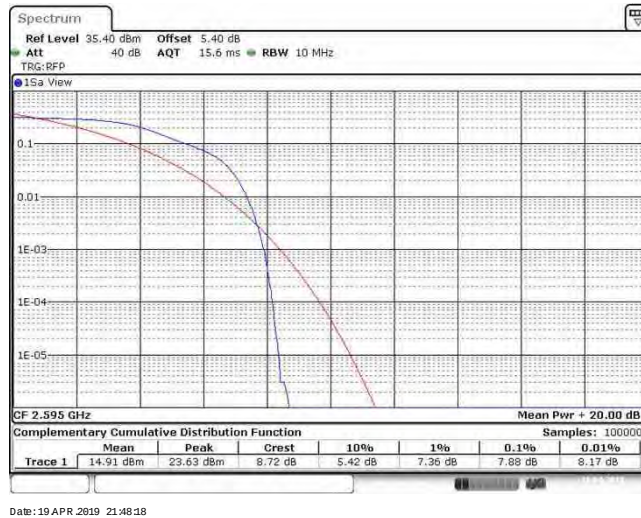
Band38_20MHz_QPSK_38150_100RB#0
