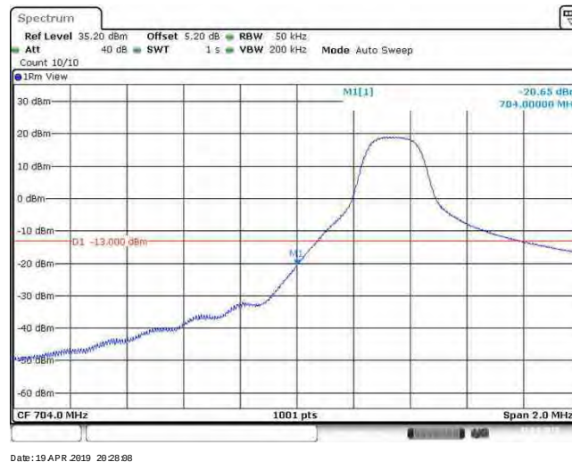
Band17_5MHz_QPSK_23755_25RB#0
