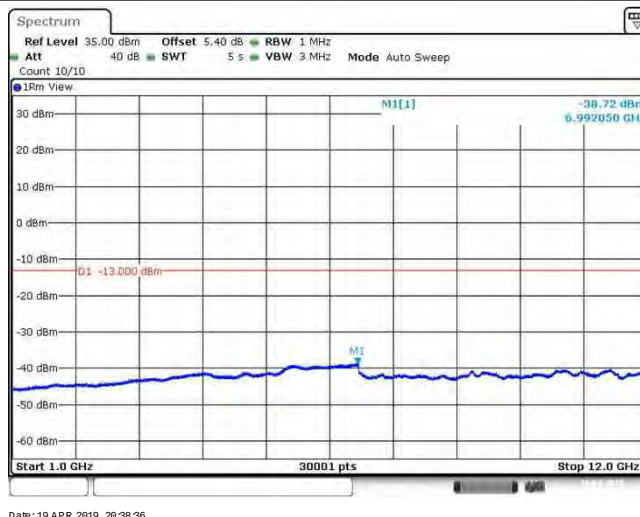
Band17_10MHz_16QAM_23790_1RB#0
