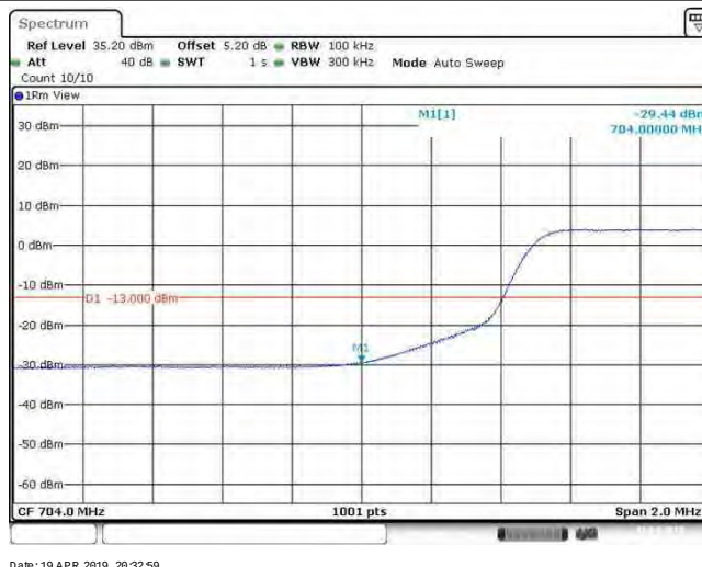
Band17_10MHz_QPSK_23800_1RB#49
