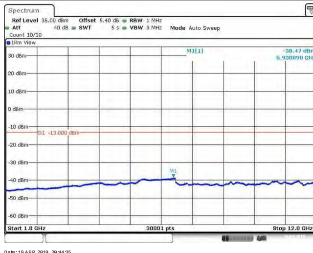
Band17_10MHz_64QAM_23800_1RB#0
