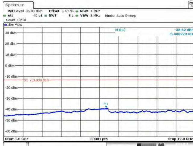
Band26_15MHz_64QAM_26915_1RB#0
