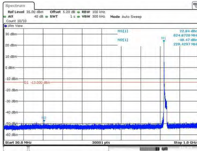
Band26_15MHz_16QAM_26865_1RB#0
