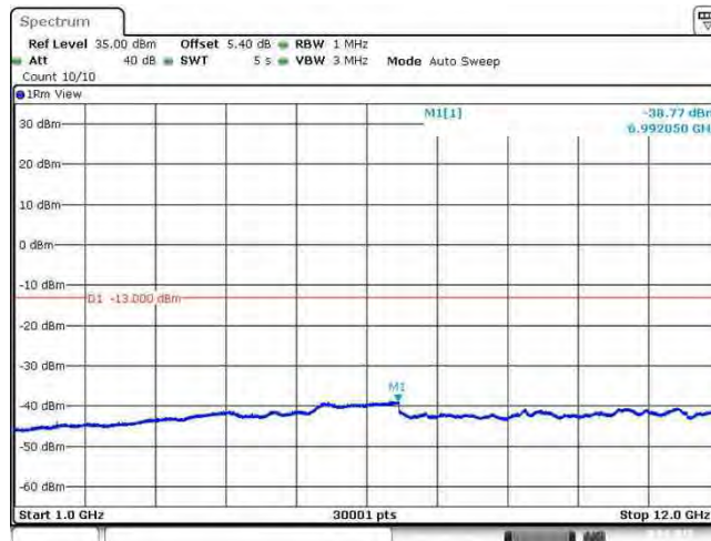
Band26_15MHz_16QAM_26865_1RB#0
