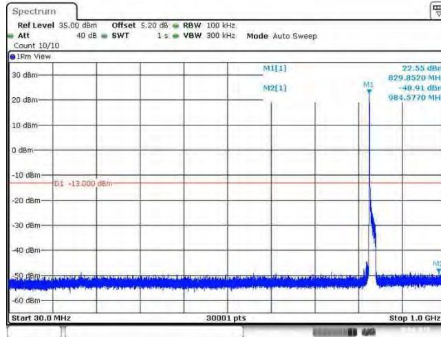
Band26_15MHz_64QAM_26915_1RB#0
