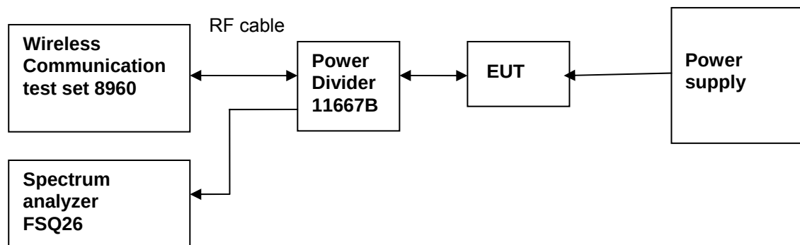
Test Set-up
