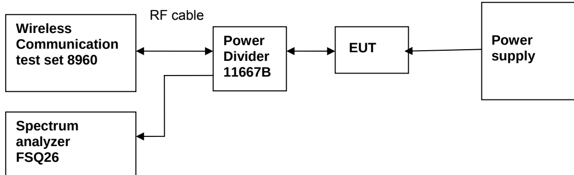
Test Set-up
