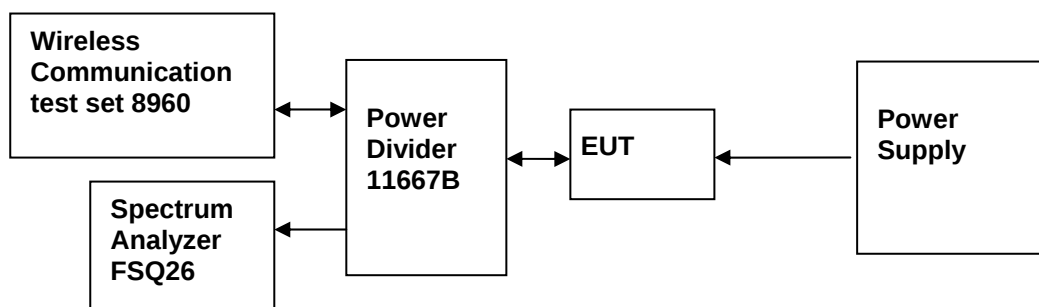
Test Set-up
