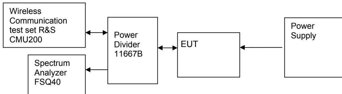
Figure 1. Test Set-up
