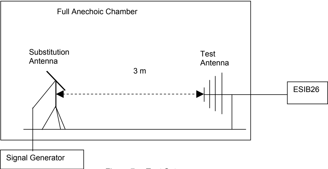
Figure 7. Test Set-up
