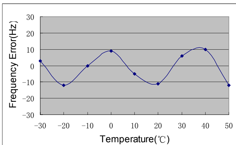
Figure 8. GPRS/GSM Mode Test Graph
