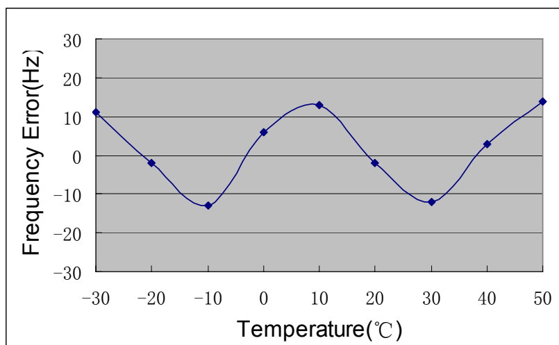
Figure 10. WCDMA Mode Test Graph
