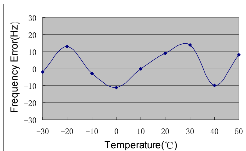
Figure 9. EDGE Mode Test Graph
