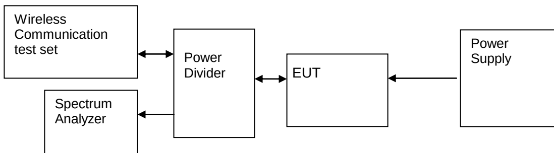
Figure 6. Test Set-up
