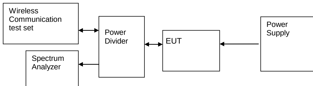
Figure 3. Test Set-up
