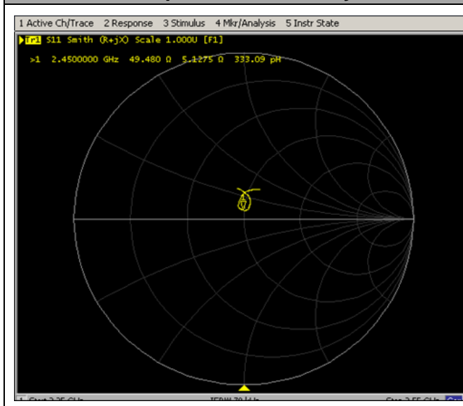
Impedance Test-Body
