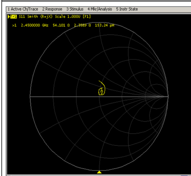
Impedance Test-Body
