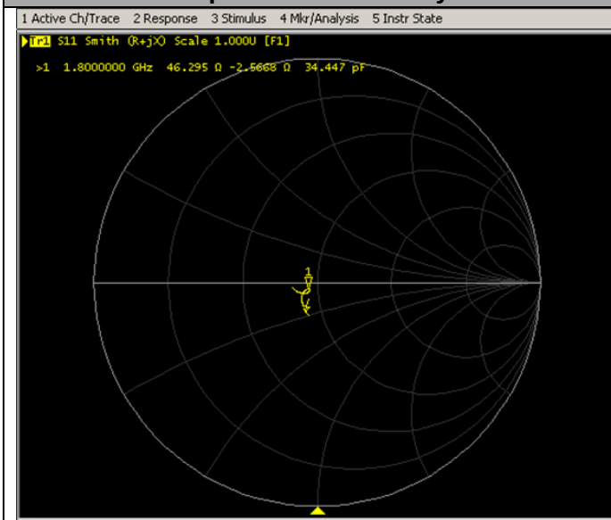
Impedance Test-Body
