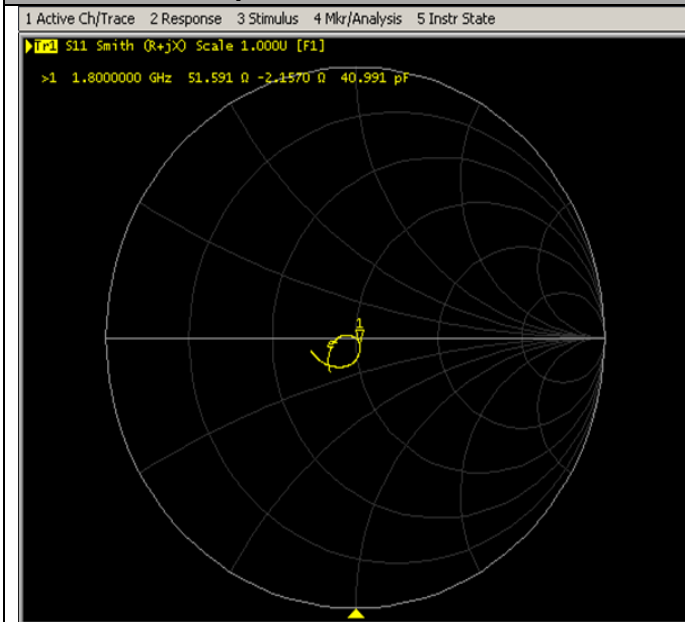
Impedance Test-Body
