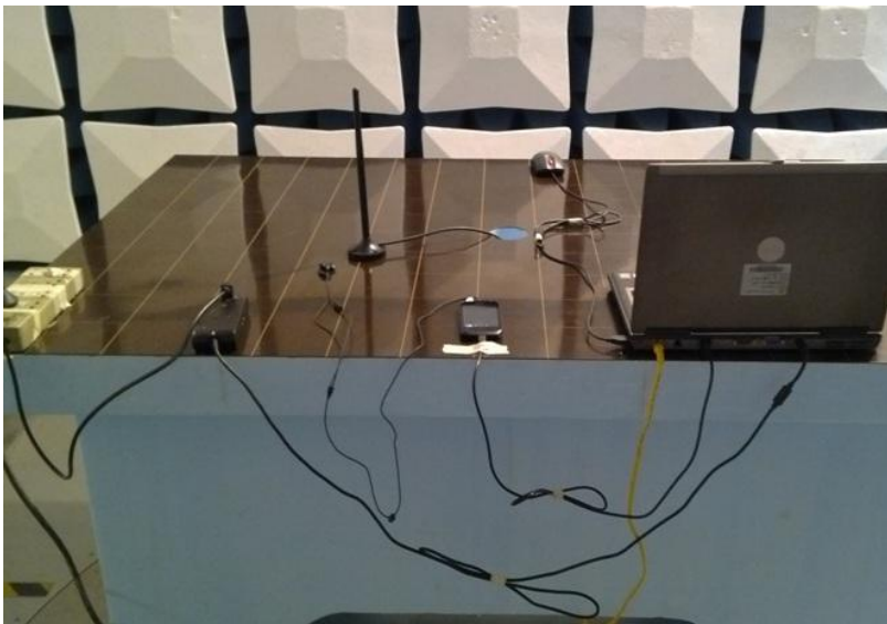
Radiated Disturbance Emissions (below 1GHz)
