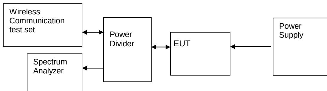
Figure 3. Test Set-up
