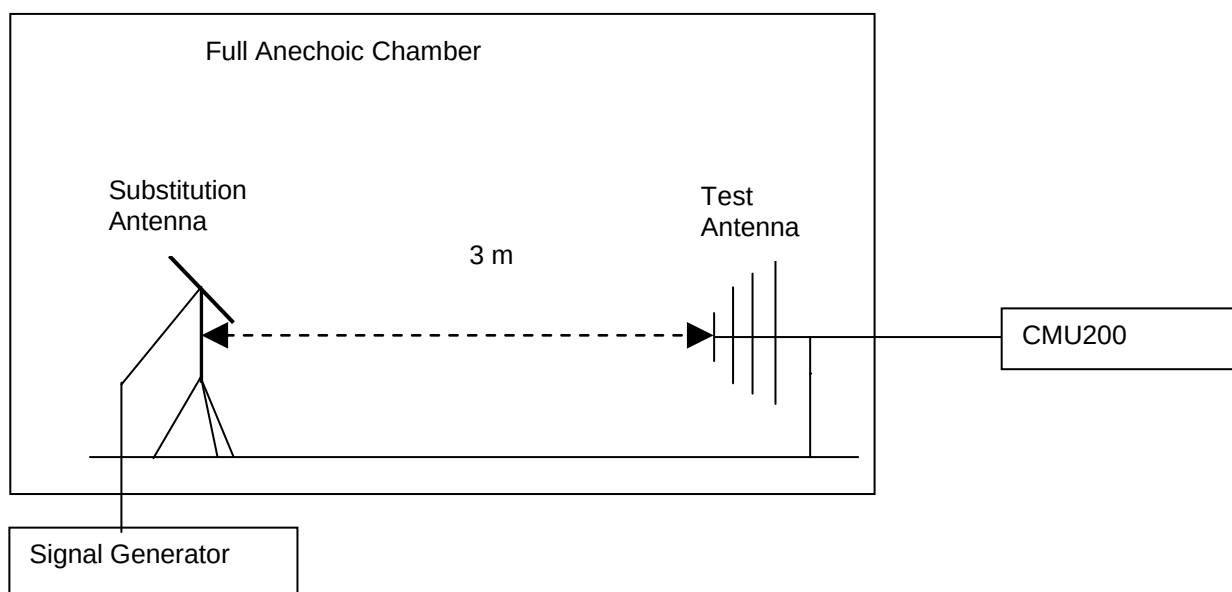
Figure 1. Test Set-up
