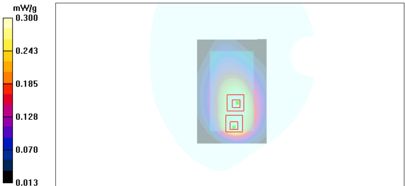
Figure 28 Body with Earphone, Towards Ground, GSM 850 Channel 251
