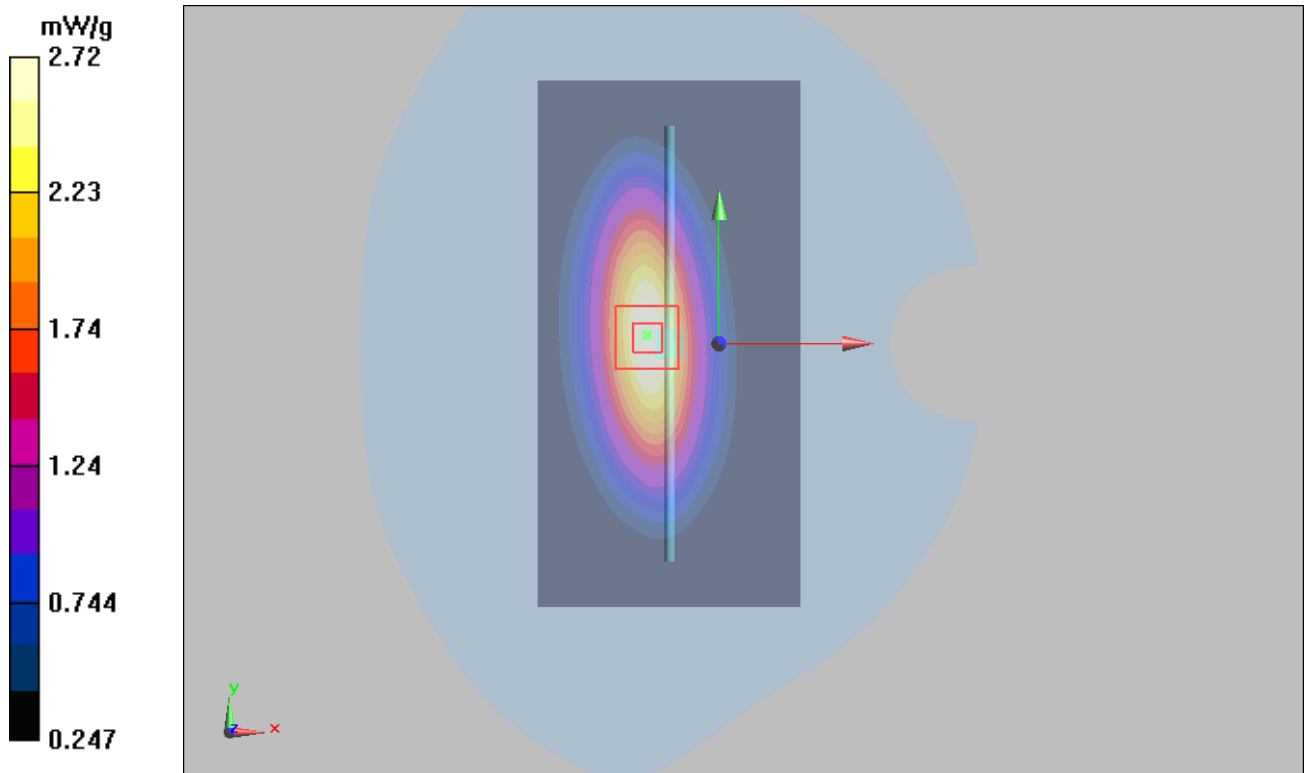
Figure 9 System Performance Check 835MHz 250mW
