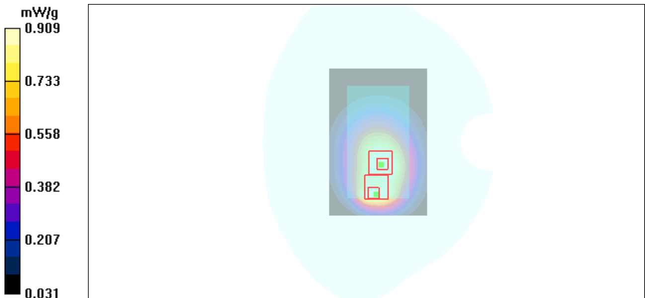
Figure 38 Body, Towards Ground, GSM 850 EGPRS(2TXslots) Channel 251
