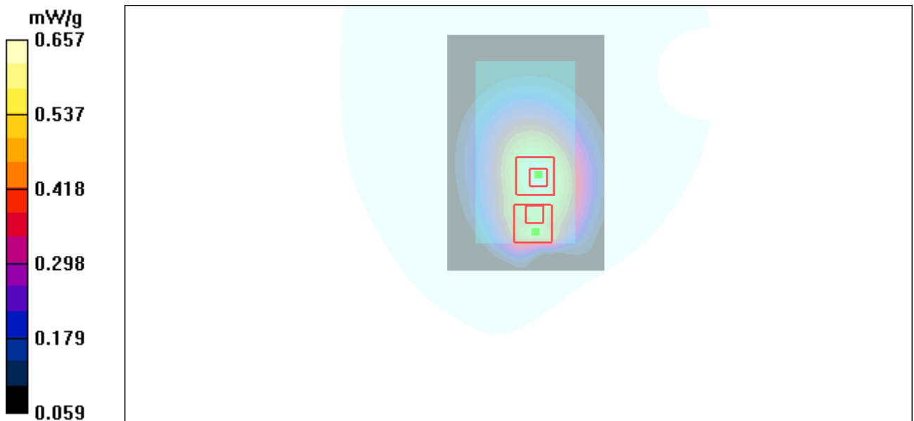
Figure 24 Body, Towards Ground, GSM 850 GPRS(2TXslots) Channel 251
