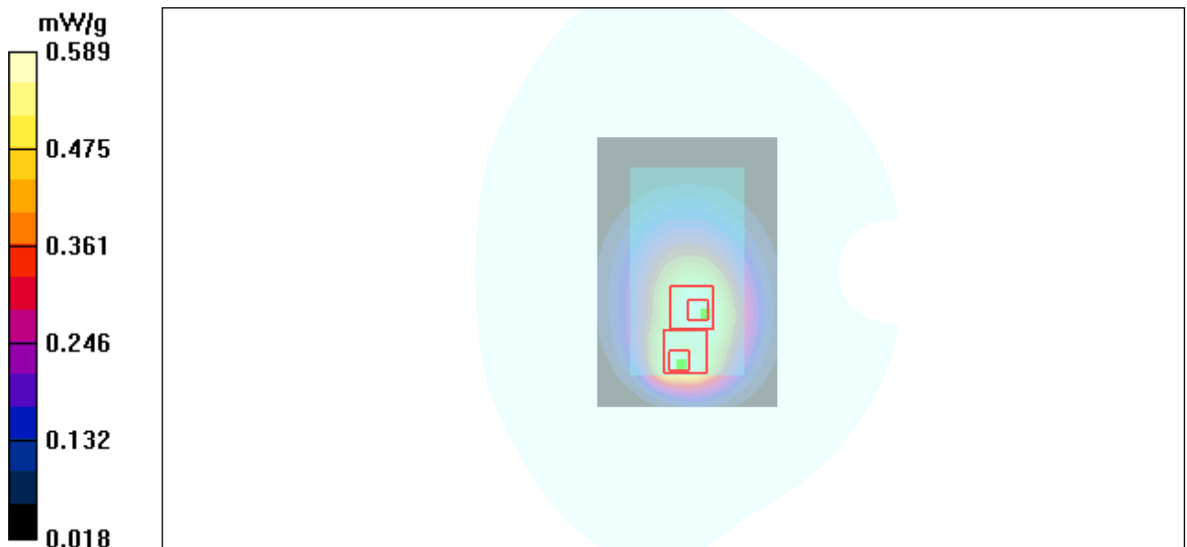
Figure 33 Body, Towards Ground, GSM 850 GPRS(2TXslots) Channel 128
