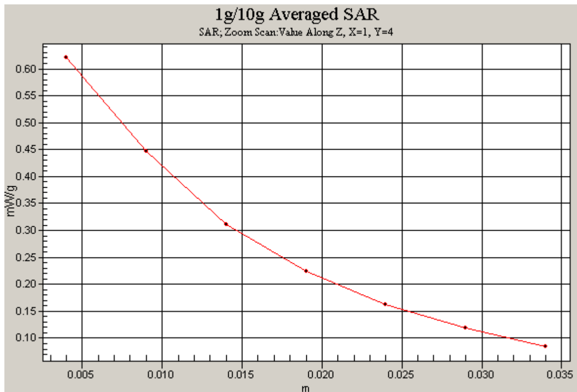
Figure 30 Body, Towards Ground, GSM 850 GPRS(2TXslots) Channel 251
