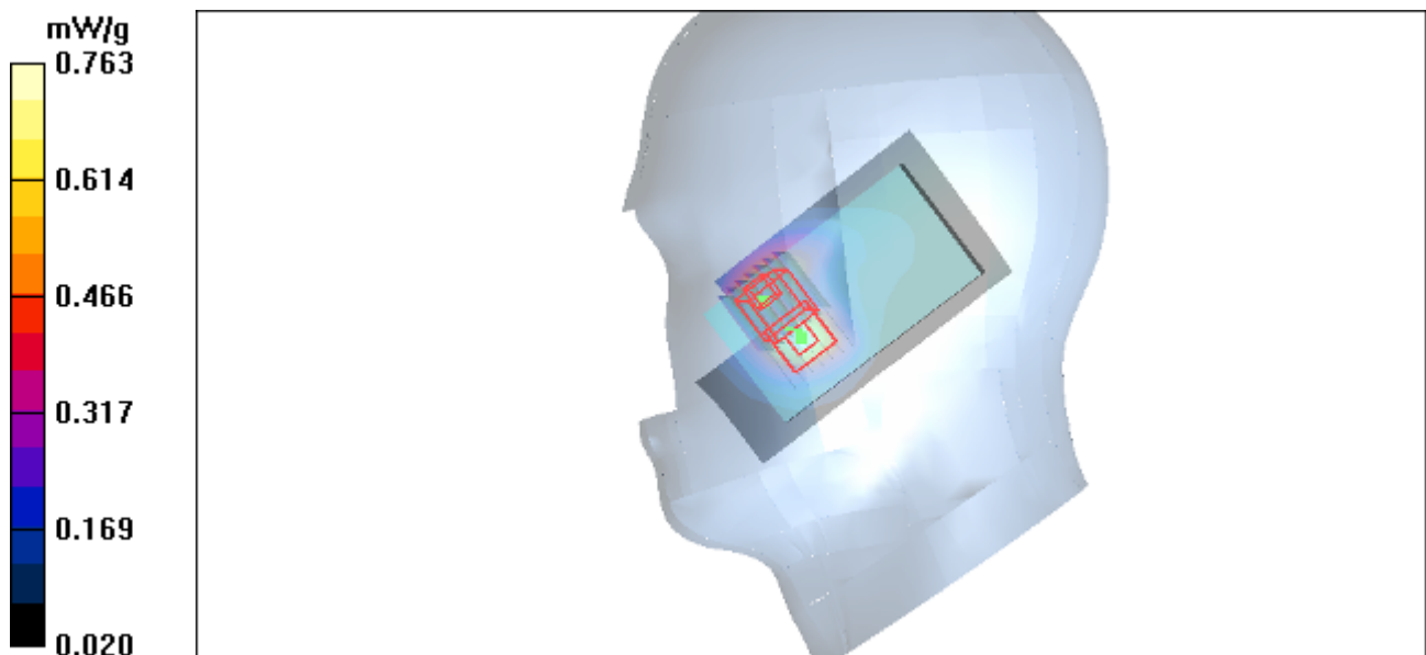
Figure 47 Right Hand Touch Cheek GSM 1900 Channel 661
