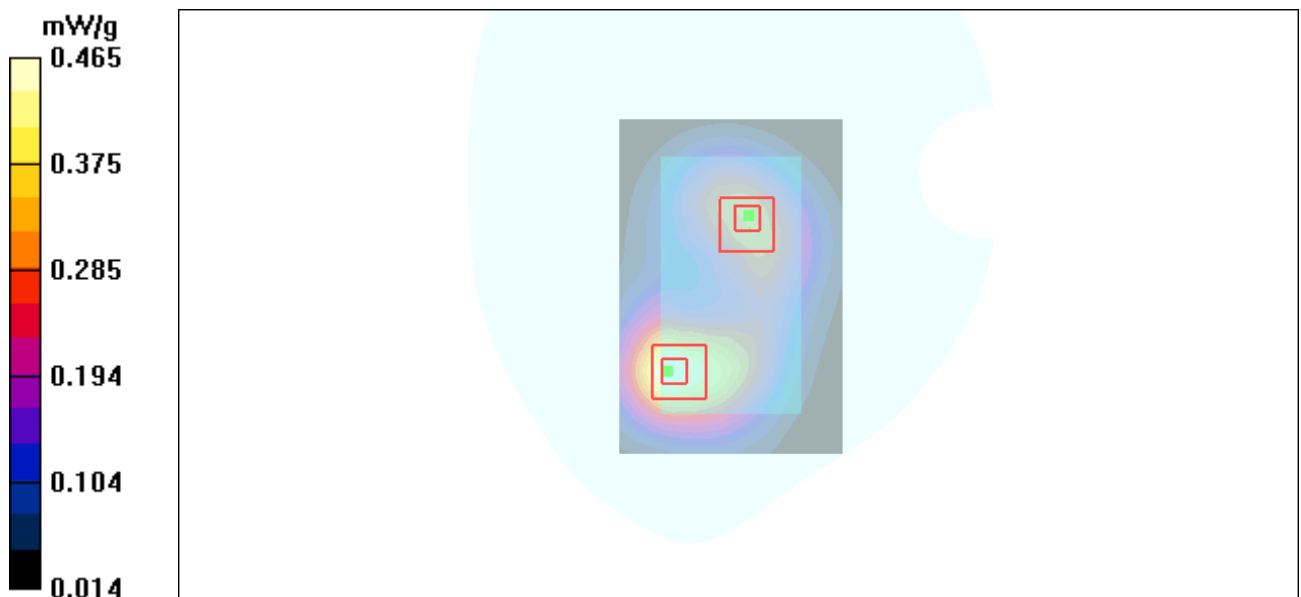
Figure 54 Body, Towards Phantom, GSM 1900 GPRS(2TXslots) Channel 661
