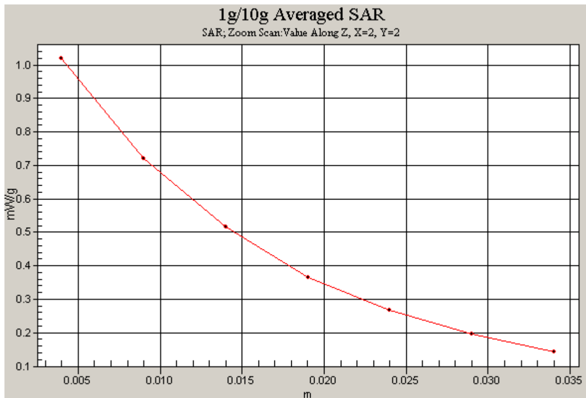
Figure 31 Body, Towards Ground, GSM 850 GPRS(2TXslots) Channel 251
