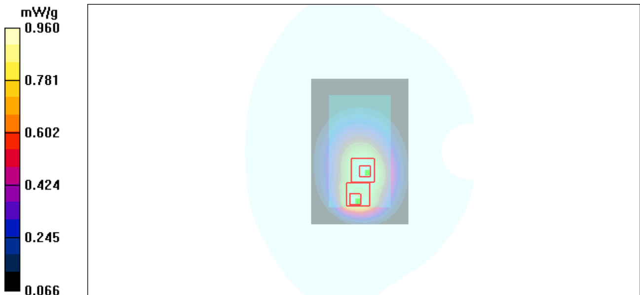
Figure 39 Body, Towards Ground, GSM 850 GPRS(2TXslots) Channel 251
