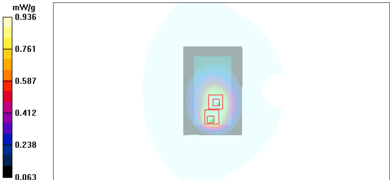
Figure 32 Body, Towards Ground, GSM 850 GPRS(2TXslots) Channel 190
