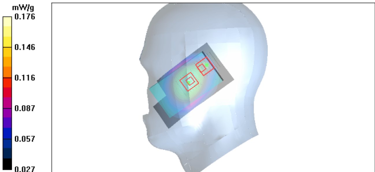
Figure 21 Right Hand Tilt 15° GSM 850 Channel 190
