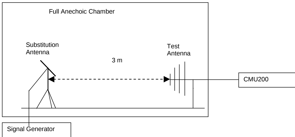
Figure 1. Test Set-up
