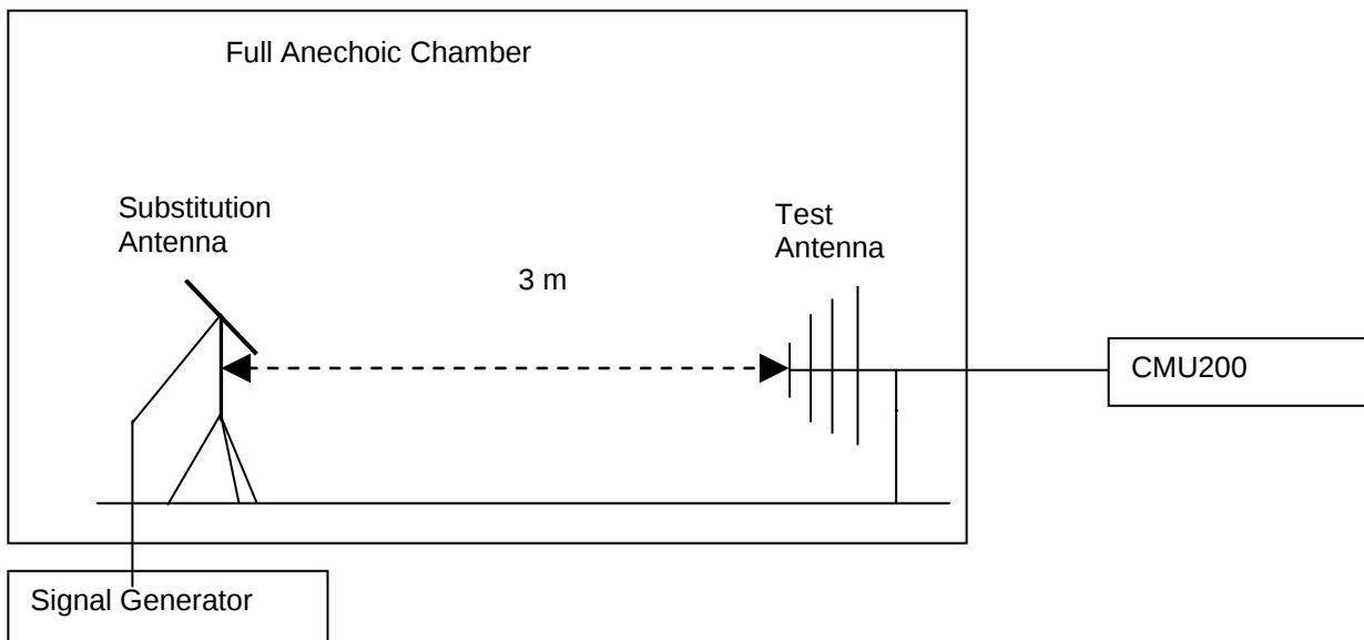
Figure 1. Test Set-up
