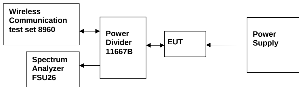
Test Set-up
