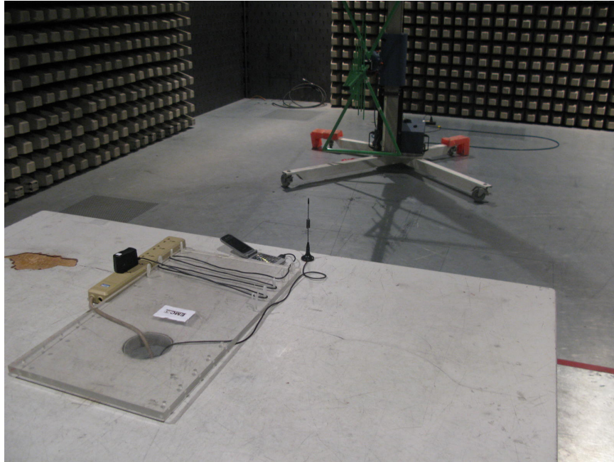
Radiated Disturbance
