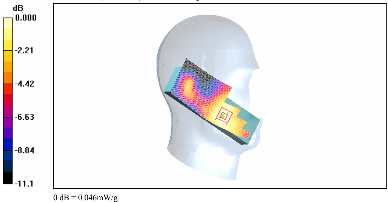
Fig. 7 Left Hand Tilt 15° PCS 1900MHz CH810
