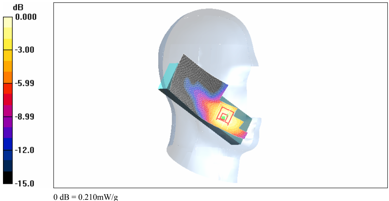
Fig. 5 Left Hand Touch Cheek PCS 1900MHz CH512
