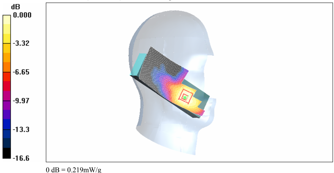
Fig. 3 Left Hand Touch Cheek PCS 1900MHz CH661
