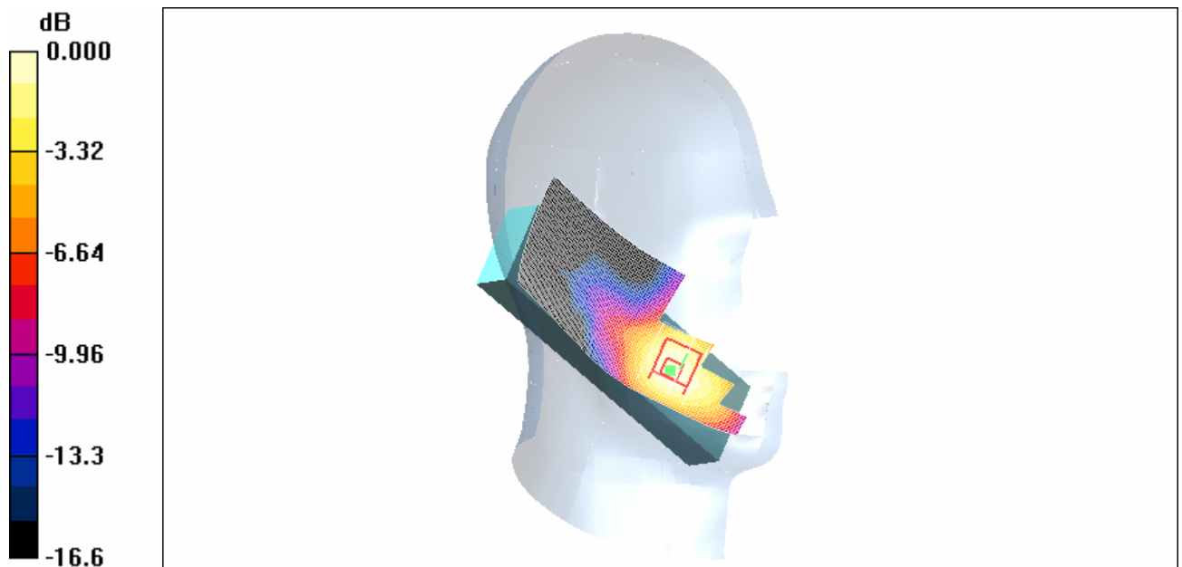
Fig. 1 Left Hand Touch Cheek PCS 1900MHz CH810
