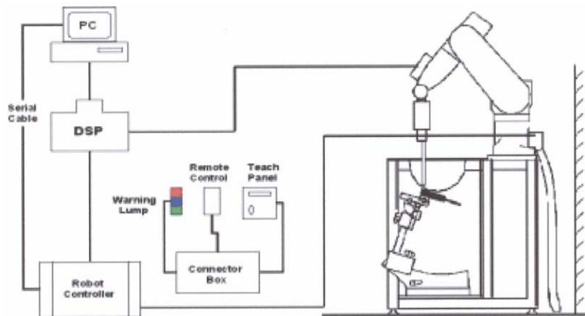
Picture 1: SAR Lab Test Measurement Set-up
