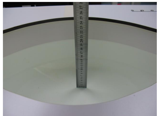
Photo 17:MSL 1900MHz depth (15.1cm)
