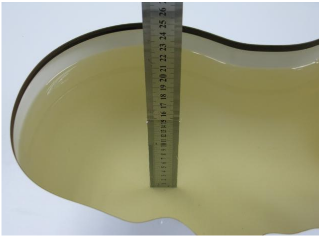
Photo 14:HSL 1800MHz depth (15.3cm)
