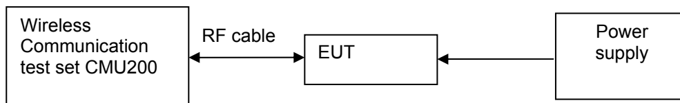
Figure 7. Test Set-up
