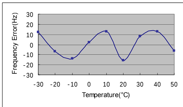
Figure 8. WCDMA Mode Test Graph
