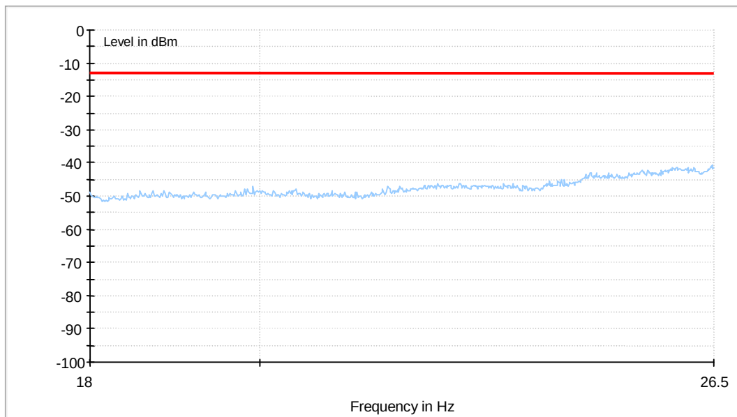
Figure 7. Radiated Spurious Emission
