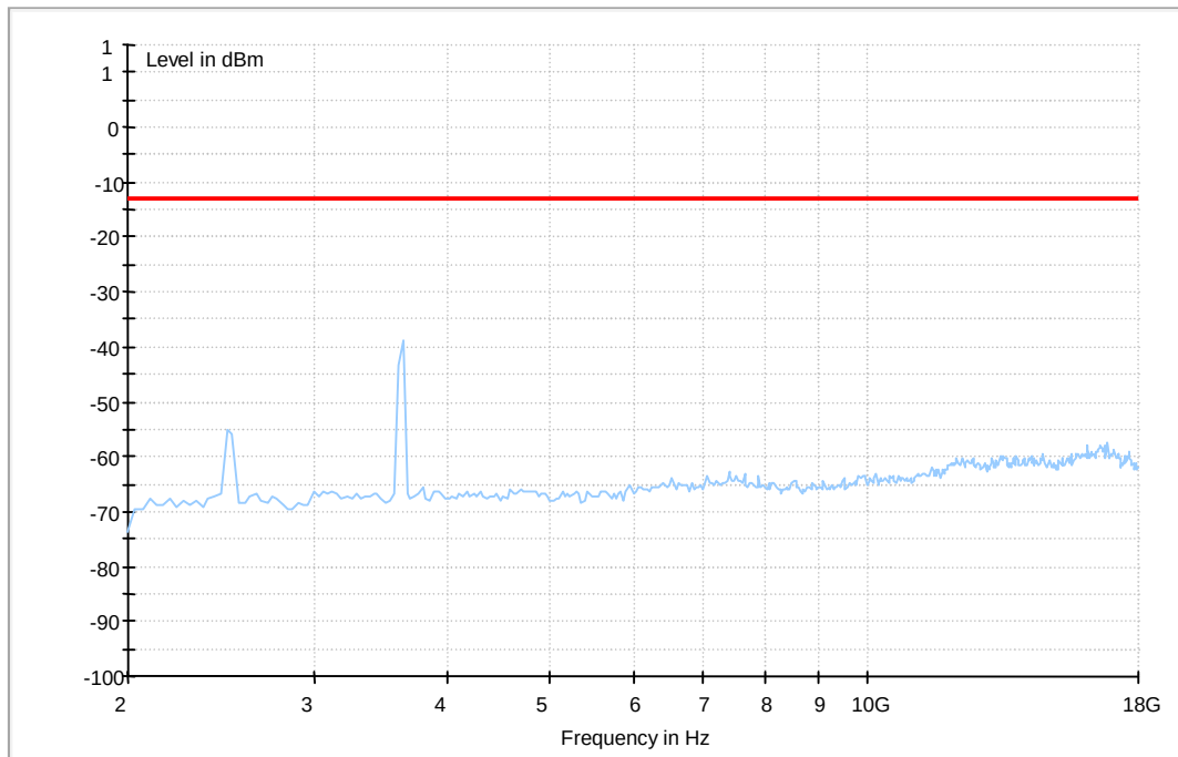
Figure 8. Radiated Spurious Emission
