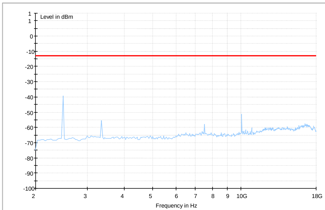
Figure 5. Radiated Spurious Emission
