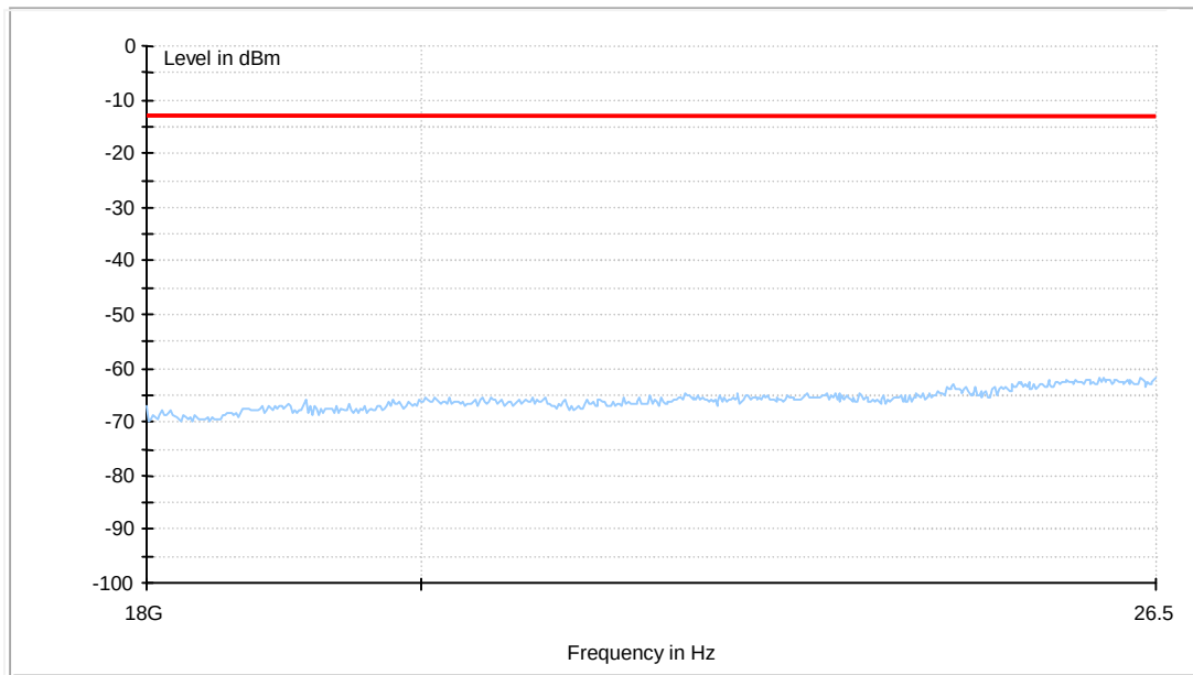
Figure 9. Radiated Spurious Emission
