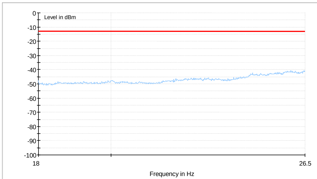
Figure 6. Radiated Spurious Emission
