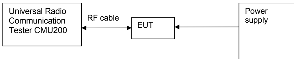
Figure 2. Test Set-up
