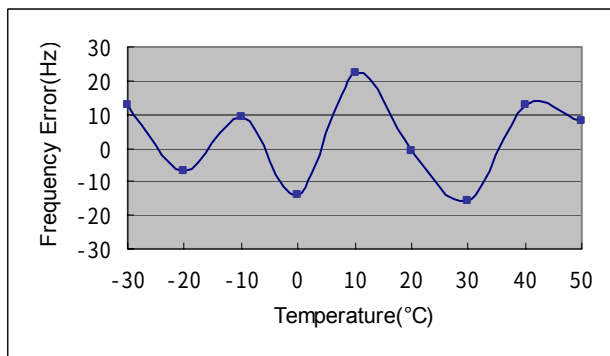
Figure 9. TM2 Test Graph
