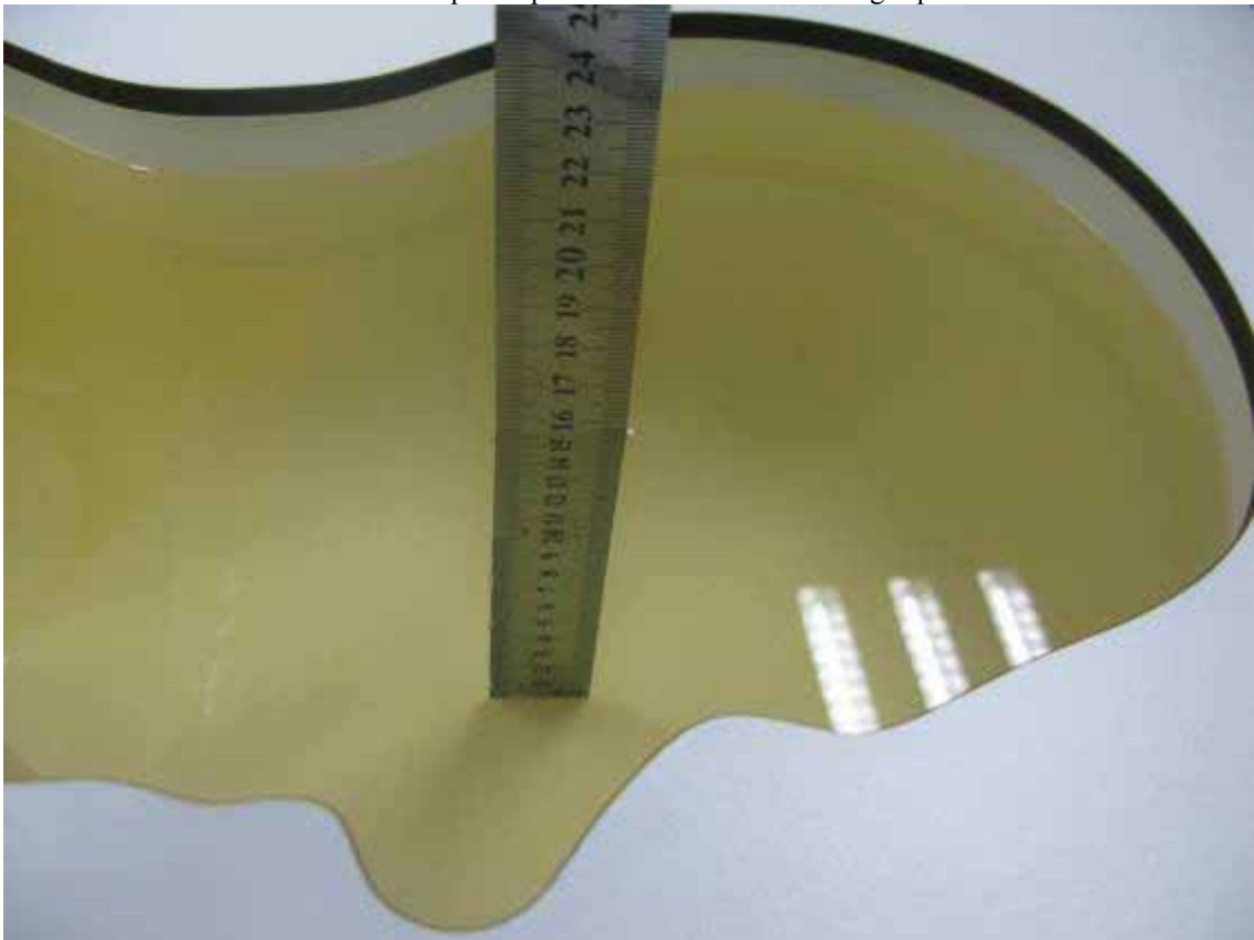
Photo 13: Liquid depth 900 MHz head simulating liquid
