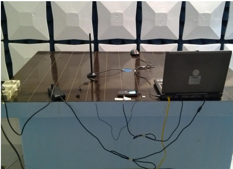
Radiated Spurious Emission (below 1GHz)
