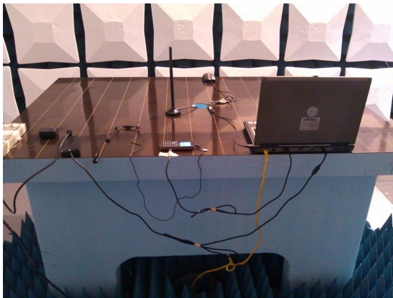
Radiated Disturbance (1GHz to18GHz)
