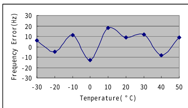
Figure 9. EDGE Mode Test Graph
