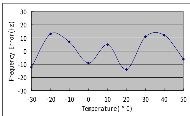
Figure 8. GPRS/GSM Mode Test Graph
