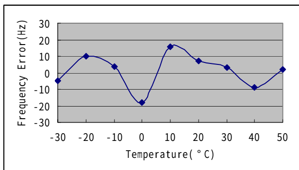
Figure 10. WCDMA Mode Test Graph
