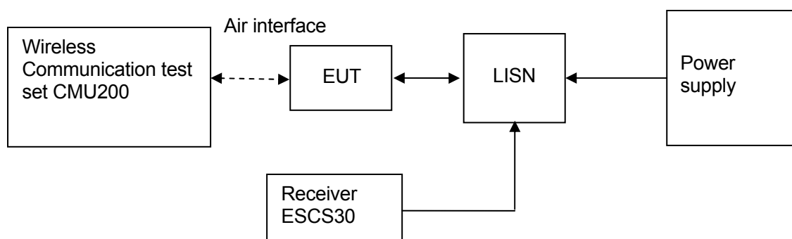
Figure 4. Test Set-up
