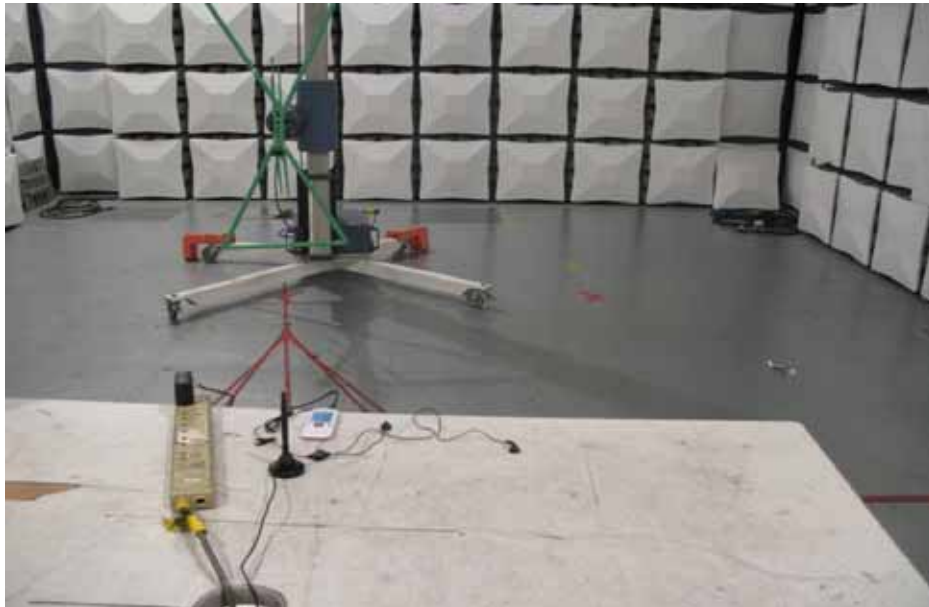
Radiated Spurious Emission (below 2GHz)
