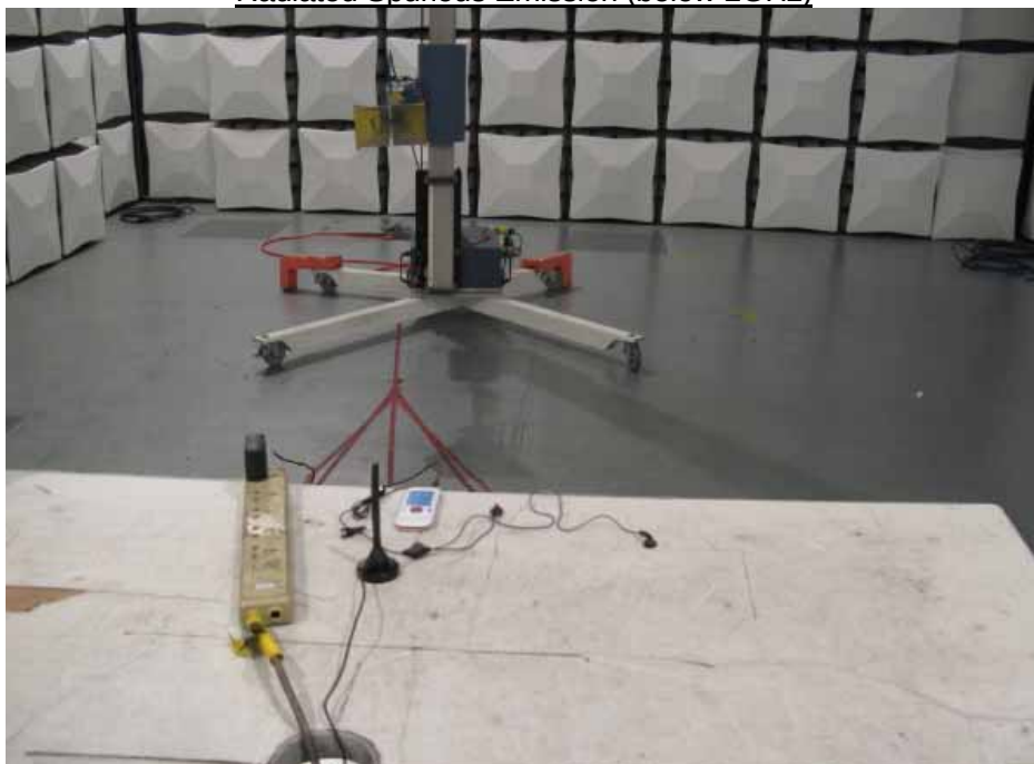
Radiated Spurious Emission (2GHz to18GHz)
