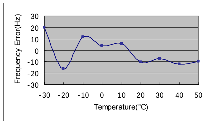
Figure 10. WCDMA Mode Test Graph
