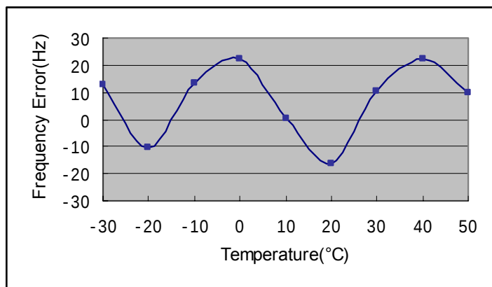
Figure 8. GPRS/GSM Mode Test Graph
