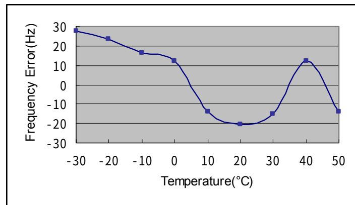
Figure 10. TM3 Test Graph
