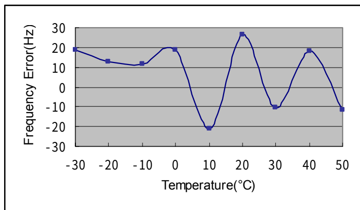
Figure 8. TM1 Test Graph
