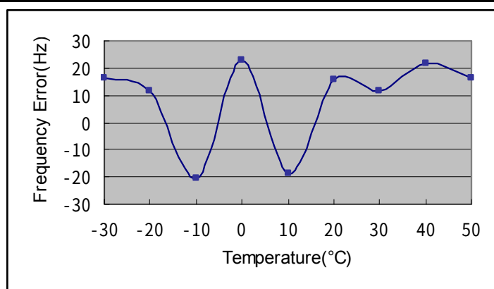
Figure 9. TM2 Test Graph
