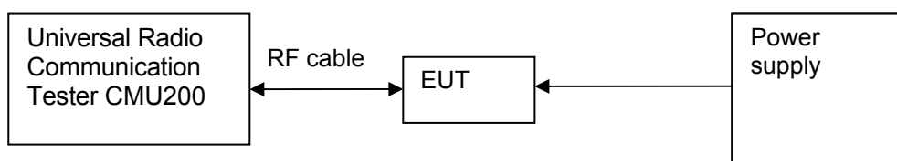
Figure 3. Test Set-up
