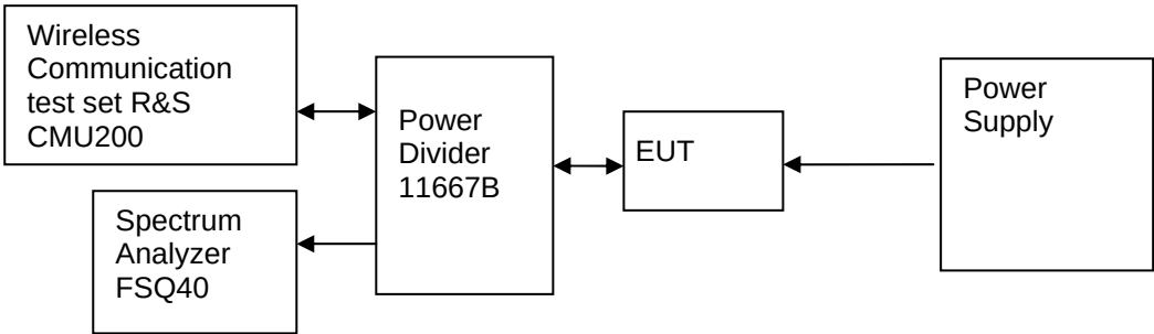
Figure 2. Test Set-up
