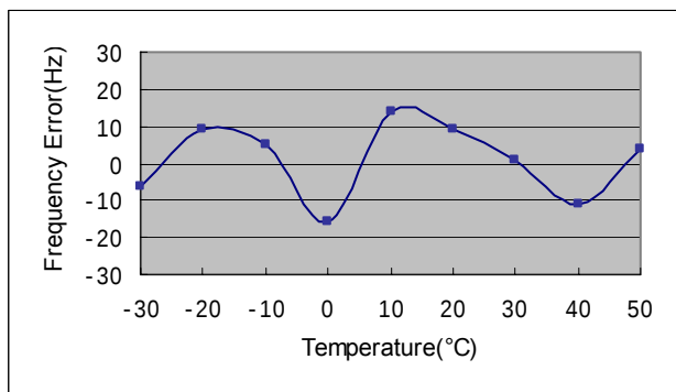
Figure 9. WCDMA Mode Test Graph
