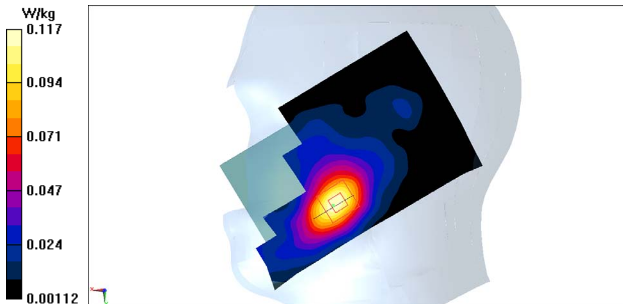
Fig.3 1900 MHz
