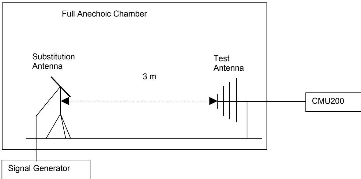
Figure 1. Test Set-up
