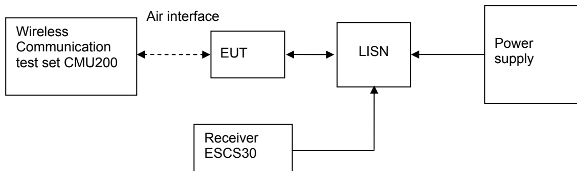
Figure 10. Test Set-up
