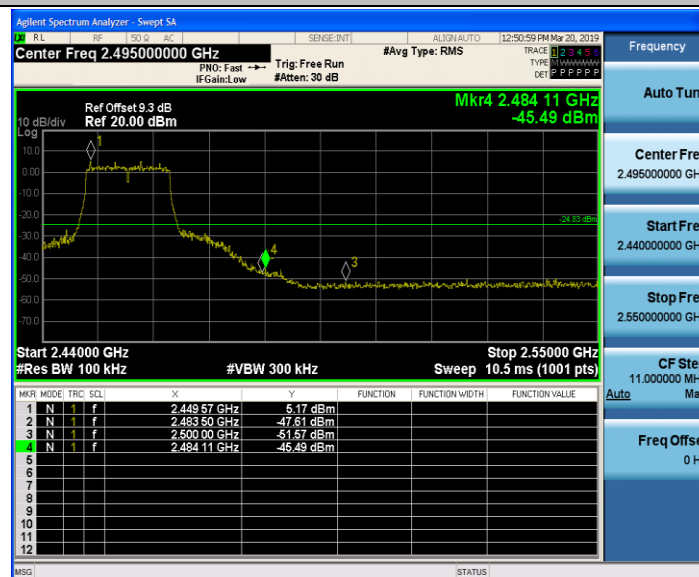
11G_Ant1_High_2457
