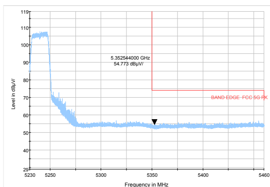
802.11a-Channel 48: Average
