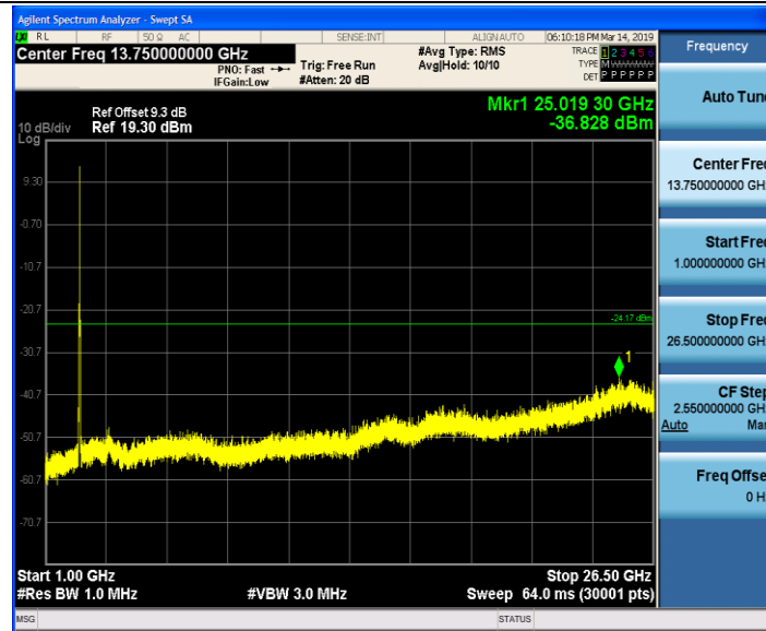
11G_Ant1_2457_0~Reference
