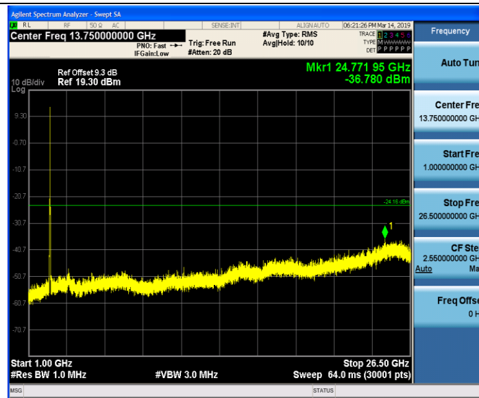
11N20SISO_Ant1_2457_0-Reference
