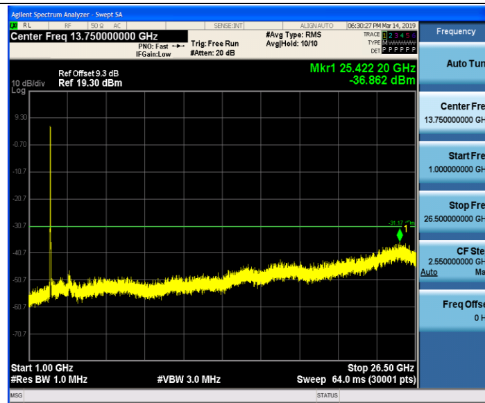
11N40SISO_Ant1_2427_0-Reference
