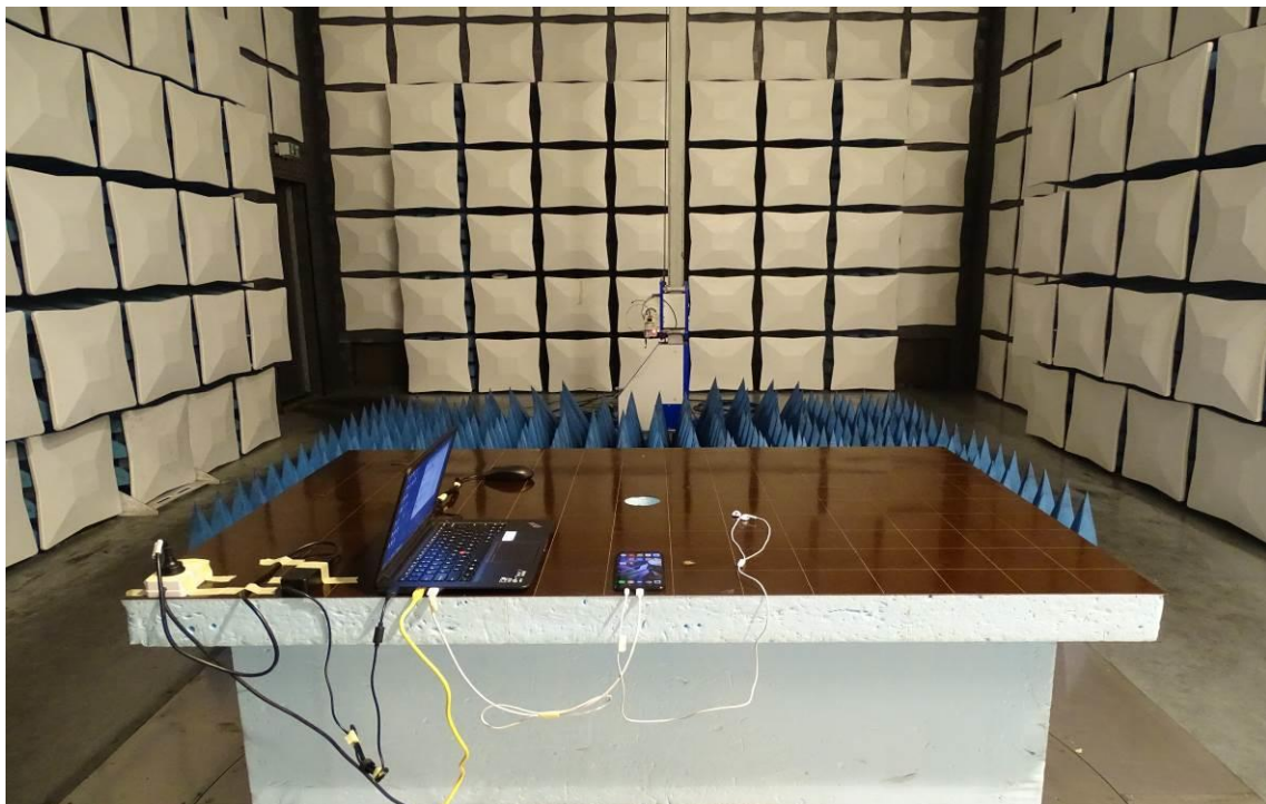
Radiated Disturbance Emissions (26.5GHz to 40GHz)
