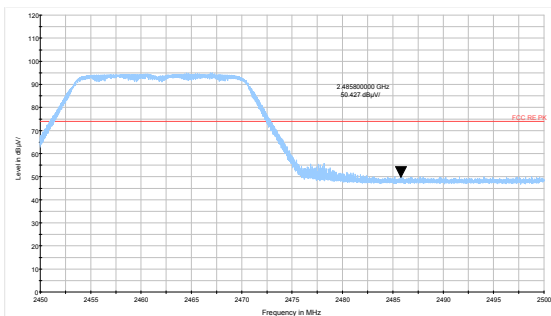
802.11b-Channel 11 Peak
