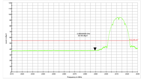
802.11b-Channel 1 Average
