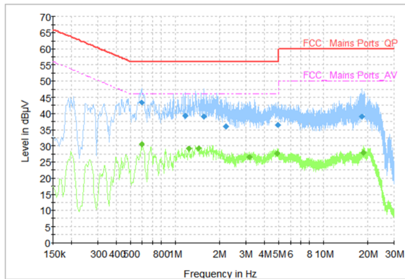
Fig.28 AC Power line Conducted Emission (Idle, AE1, 120V)
