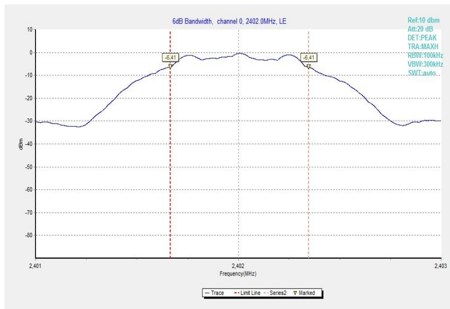
Fig.4 Occupied 6dB Bandwidth (Ch 0)
