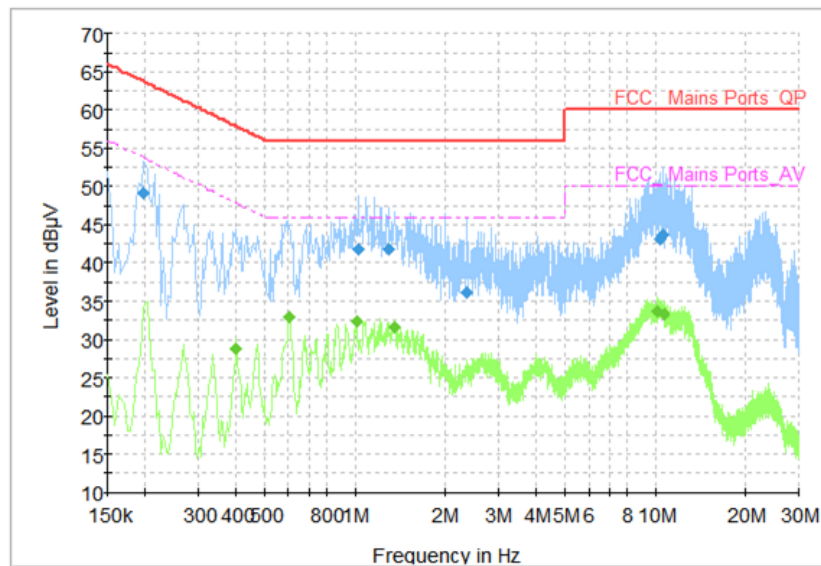
Fig.30 AC Power line Conducted Emission (Idle, AE2, 120V)
