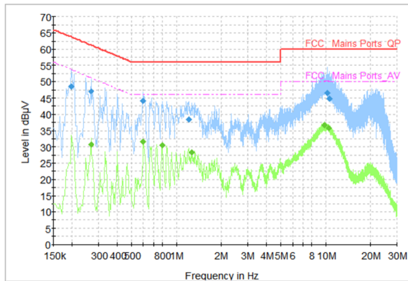
Fig.36 AC Power line Conducted Emission (Idle, AE2, 240V)
