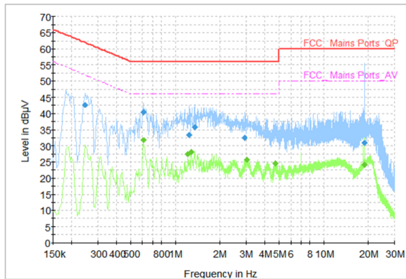
Fig.34 AC Power line Conducted Emission (Idle, AE1, 240V)
