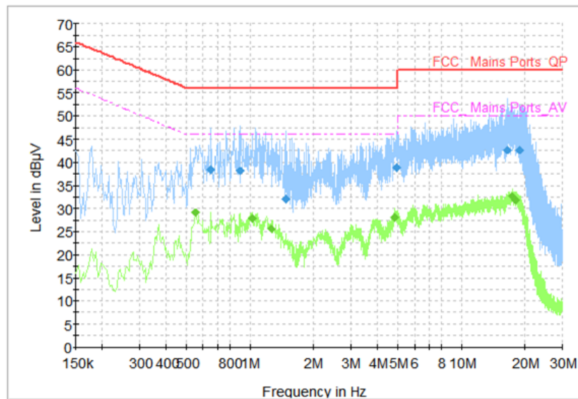
Fig.38 AC Power line Conducted Emission (Idle, AE3, 240V)
