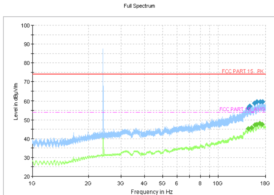
Fig.19 Radiated Spurious Emission (GFSK, Ch0, 1 GHz ~18 GHz)
