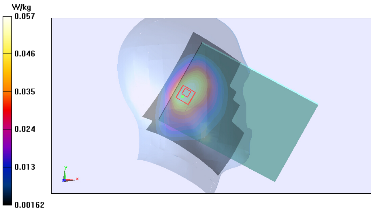
Figure 56 Left Hand Tilt 15° UMTS Band IV Channel 1413
