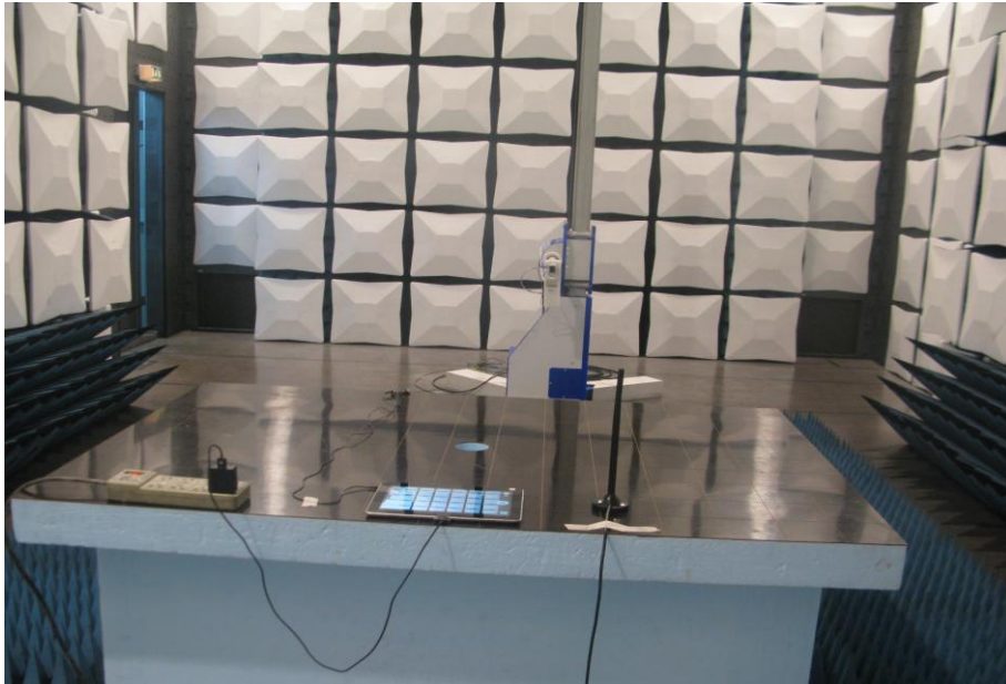
Radiated Spurious Emission (above 18GHz)
